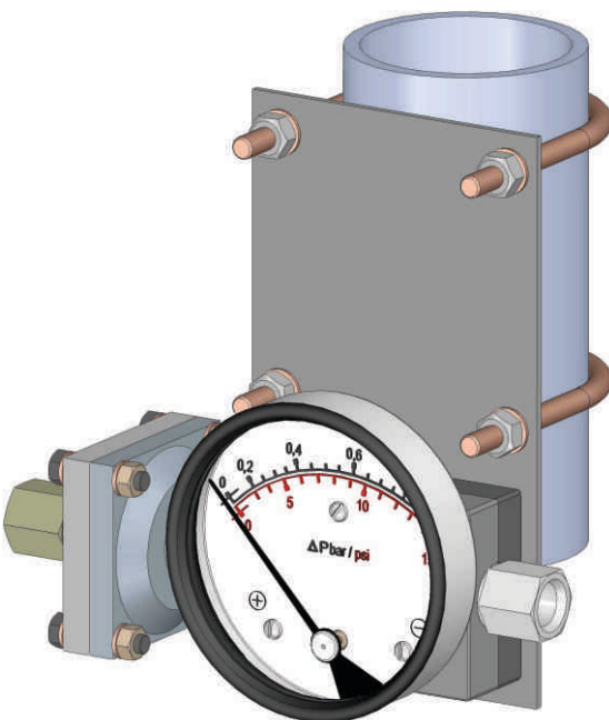
Vertical Pipe Mounting
